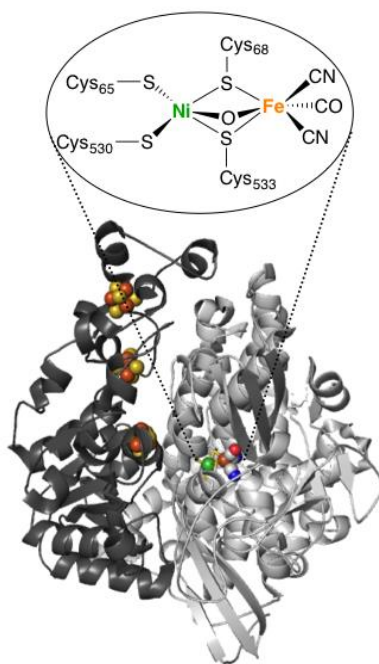
[NiFe]-hydrogenase. From the structure of the D. gigas enzyme (PDB 2FRV).
